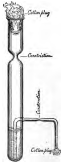
Fig. 65.—Liborius' tube for anaerobic cultures.
